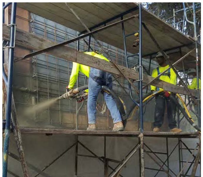
Fig. 5: Mock-up for alternative method of formwork (CROM Project Services Facility Gainesville, FL)
