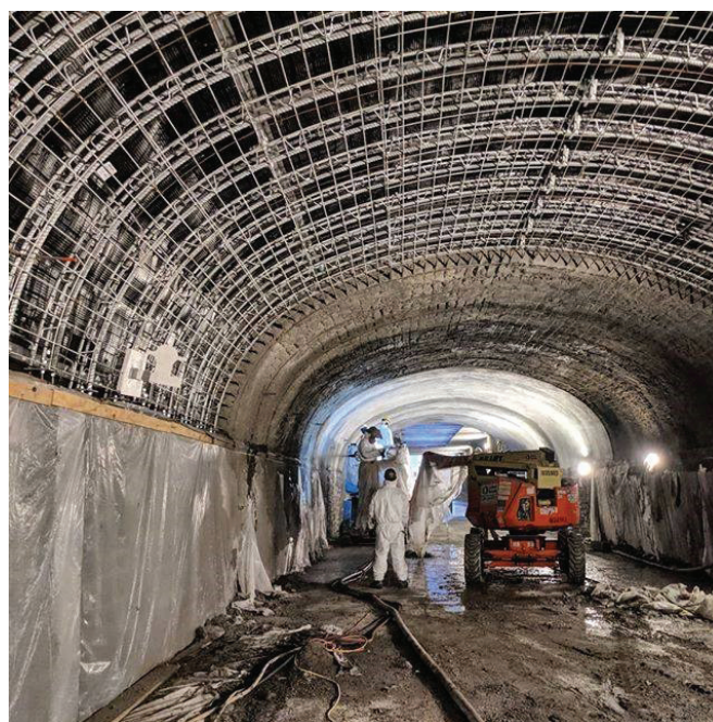
Lattice girders over waterproofing membrane, to support 9 to 12 inches of overhead shotcrete for the reconstructed ceiling arch of the Park Avenue Tunnel.
