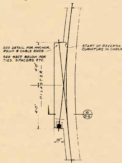
PLAN OF RING GIRDER AT PILASTER FOR CABLE ANCHORAGE
