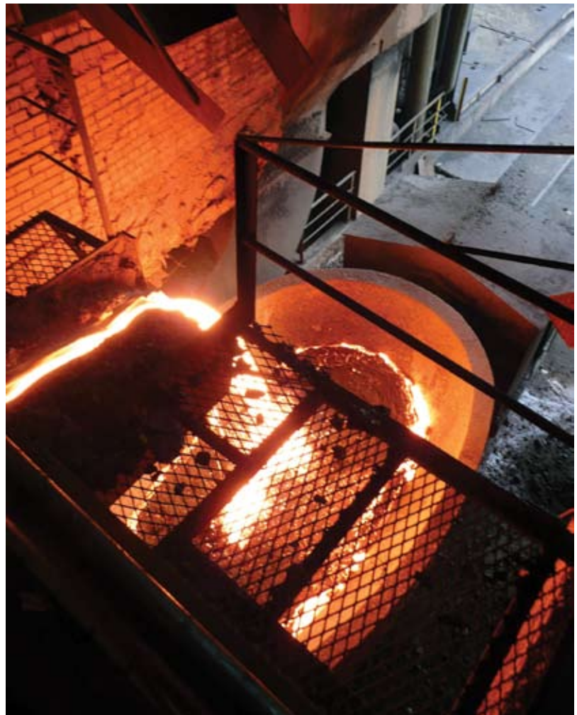
During the tap of the blast furnace, iron slag is directed into a slag pot
