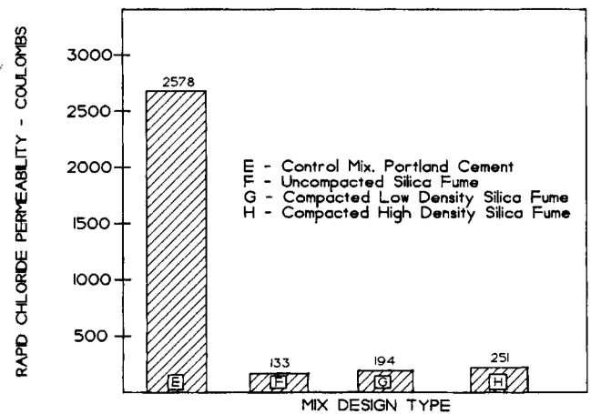
Fig. 4 — Rapid chloride permeability of dry-mix shotcrete.
