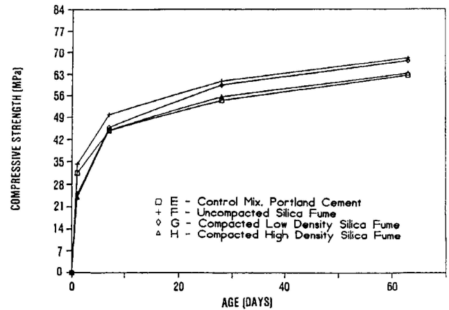
Fig. 2 — Compressive strength of dry-mix shotcrete.
