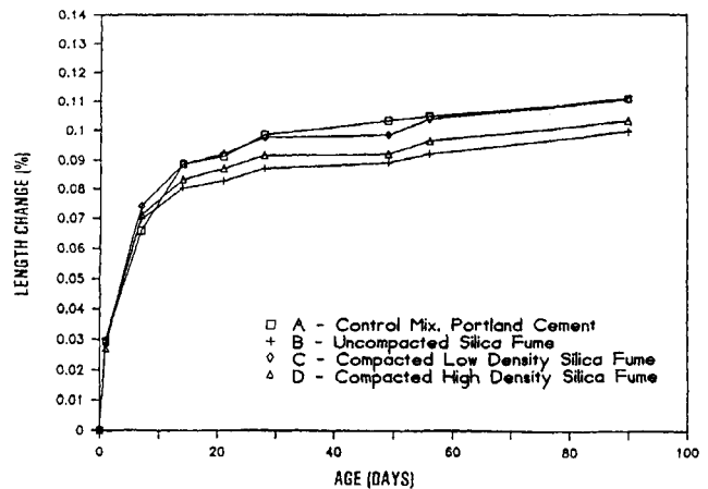
Fig. 7 — Drying shrinkage of wet-mix shotcrete.
