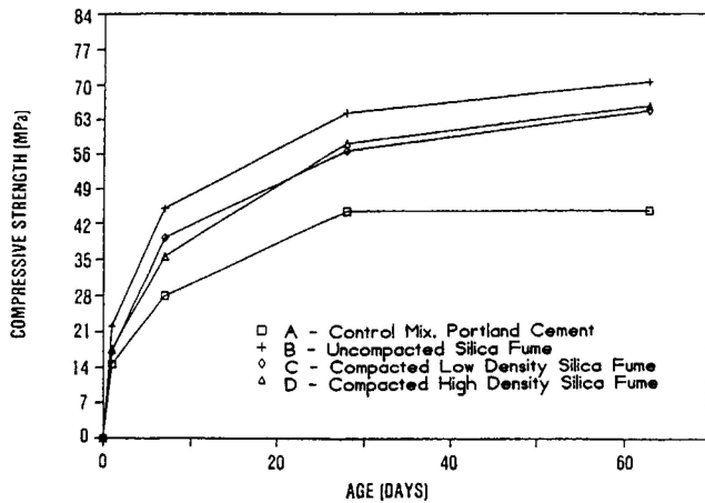
Fig. 1 — Compressive strength of wet-mix shotcrete.
