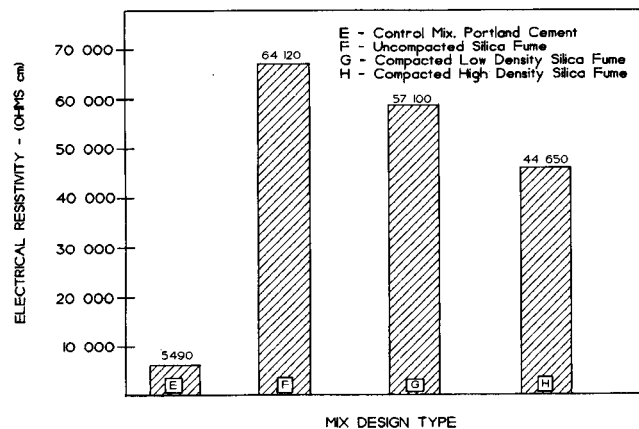
Fig. 6 — Electrical resistivity of dry-mix shotcrete.
