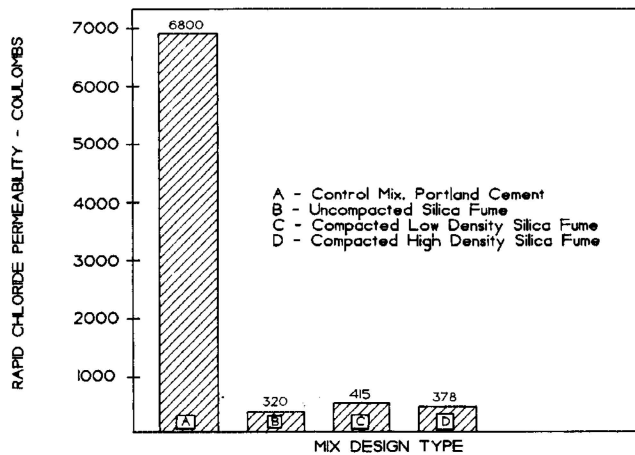
Fig. 3 — Rapid chloride permeability of wet-mix shotcrete.
