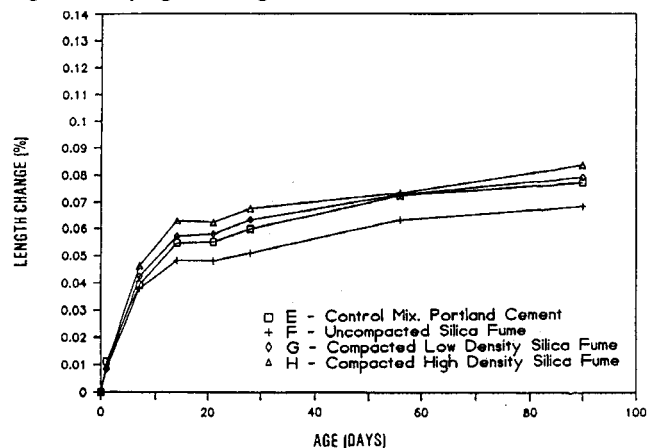
Fig. 8 — Drying shrinkage of dry-mix shotcrete.
