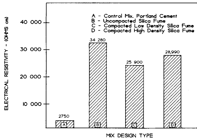
Fig. 5 — Electrical resistivity of wet-mix shotcrete.
